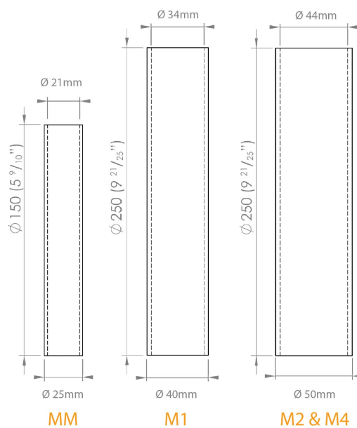
Outer Diameters
