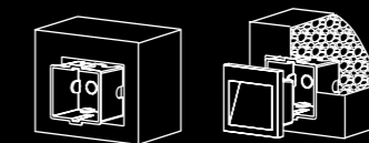
PVC WALL BOX
