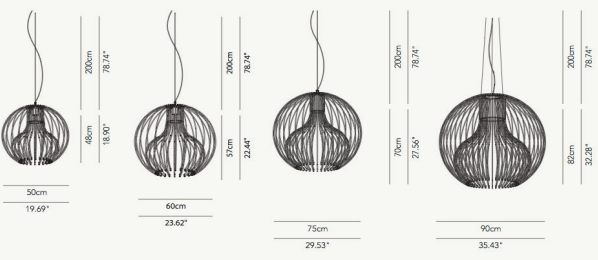
Product Name: Icaro Ball Designer: Brian Rasmussen Manufacturer: Modo IP: 65 Light Source: LED E27 or Fluorescent 1 x 20W E27 Material: Steel Wire Finishes: Black, Natural or White
