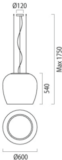
Product Name: Hand Made Designer: Sandro Santantonio Design Manufacturer: Modo IP: 44 Light Source: E27 3x30W TC-TSE Material: Natural Fiberglass Finishes: Natural Fiberglass
