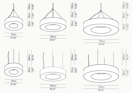
Product Name: Atollo Suspension Designer: Paolo Grasselli Manufacturer: Modo IP: 65 Light Source: LED E27 or Fluorescent 7/20W E27 Material: Polyethylene Finishes: White
