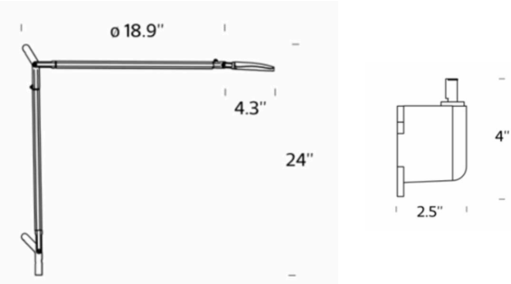
Product Name: Volee Wall Designer: Odo Fioravanti Manufacturer: Fontana Arte IP: 20 Light Source: LED - 7.5W Material: Aluminium Finishes: Flourescent Yellow, Grey or White
