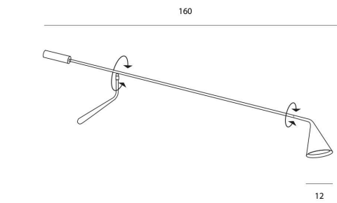
Product Name: Gordon 561.49 Designer: Corrado Dotti Manufacturer: Tooy IP: 40 Light Source: 1 x max 10W - E14 Material: Borosilicate Glass & Metal Finishes: Matte Black, Brushed Brass, Polished Gold & Black Chrome
