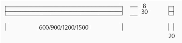
Product Name: SPINAled Mounted Designer: Daniel Kübler & Erwin Egli Manufacturer: Ribag IP: 54 Light Source: 9W, 13W, 18W or 22W Material: Aluminium & Acrylic Glass Finishes: Aluminium Matt Anodised or Aluminium Bright Chrome
