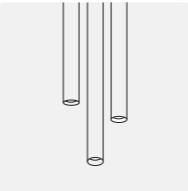
Cluster
