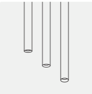
Cascading
