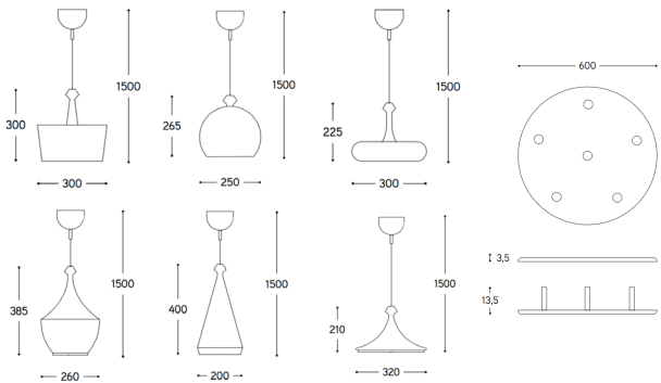
Product Name: L7 Multilustri Designer: Aldo Bernardi Manufacturer: Aldo Bernardi IP: 20 Light Source: E27 or LED Material: Ceramic Finishes: Refer to product on the website
