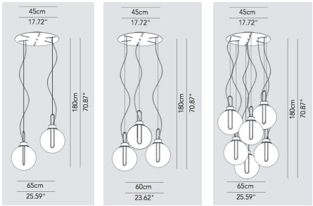
Product Name: Orb 2L / 3L / 6L Designer: Büro Famos Manufacturer: Modo IP: 20 Light Source: 1 x LED 7W 3000K Material: PMMA/Metal Finishes: White, Black, Chrome, Copper or Brass
