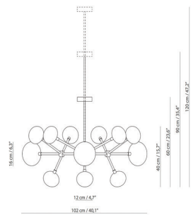
Product Name: Nabila Designer: Corrado Dotti Designer Manufacturer: Tooy IP: 20 Light Source: 12 x MAX 25W - G9 Material: Borosilicate glass | Metal Finishes: Black and Brushed Brass
