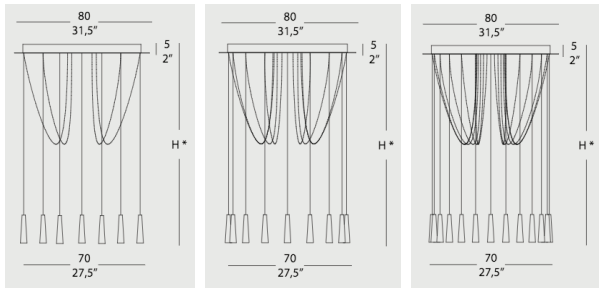
Product Name: Santral LA8 / LA16 / LA24 Designer: Filippo Mambretti Manufacturer: Morosini IP: 20 Light Source: LED 3,1W (3000K, CRI>80) Material: Aluminium with Satin Finishes: Matt Black
