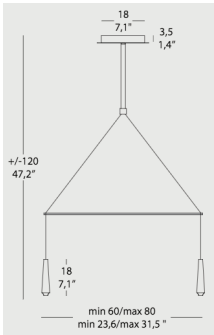
Product Name: Mikado S2L Designer: Filippo Mambretti Manufacturer: Morisini IP: 20 Light Source: LED 2 x 3.1W 3000K Material: Aluminium Finishes: Matt Black
