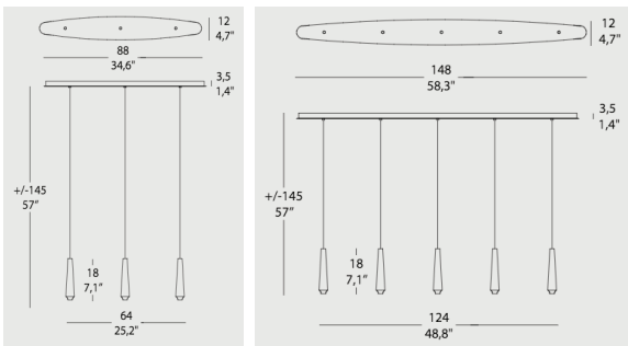
Product Name: Mikado S3L / S5L Designer: Filippo Mambretti Manufacturer: Morisini IP: 20 Light Source: LED 3.1W 3000K Material: Aluminium Finishes: Matt Black
