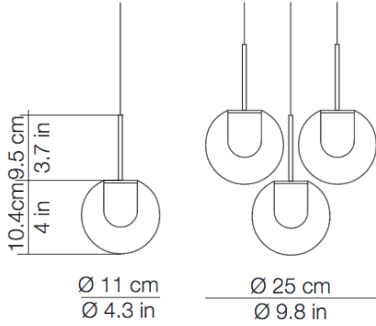
Product Name: Dew Designer: Emmanuel Babled Manufacturer: Kundalini IP: 20 Light Source: LED 4W 3000K Material: Glass Finishes: Glass
