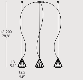
KARAT SO 3 3 x MAX 42W G9 alo. ENERGY SAVER CE F IP 20 1 ENEC
