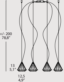
KARAT SO 4 4 x MAX 42W G9 alo. ENERGY SAVER CE F IP 20 1 ENEC
