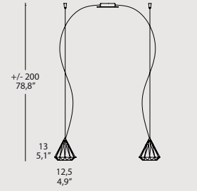
KARAT SO 2 2 x MAX 42W G9 alo. ENERGY SAVER CE F IP 20 1 ENEC
