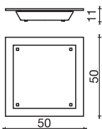
Parete/soffitto - Wall/ceiling P1 CE IP 20
