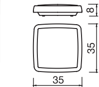
Parete/soffitto - Wall/ceiling P3 CE IP 54
