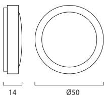
Parete/soffitto - Wall/ceiling P5
