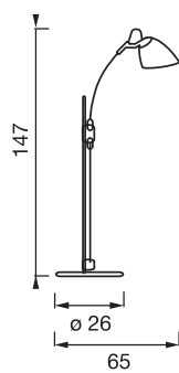
Terra - Floor TE CE IP 20
