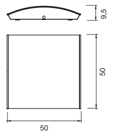
Parete/soffitto - Wall/ceiling 8 CE V IP 20
