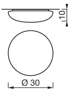
Parete/soffitto - Wall/ceiling P3 CE V A IP 44
