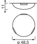
Soffitto - Ceiling P5 CE V A IP 20
