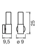
Parete - Wall A1 1x70W E27 QT-32 CE IP44
