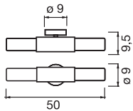
Parete - Wall A2 2x70W E27 QT-32 CE IP44
