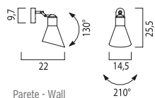
Parete - Wall CE IP 20
