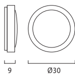
Parete/soffitto - Wall/ceiling P3 CE V A IP 54
