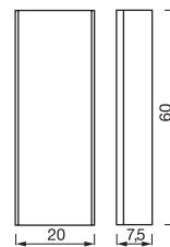
Parete/soffitto - Wall/ceiling 7 CE V IP 20
