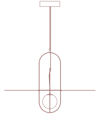
4381/1.. + disk Ø 100 cm Ø 100x54,4 +250 cm 17W (2700K, CRI>80, Lumen 2100) dimmable
