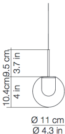
Product Name: Dew Designer: Emmanuel Babled Manufacturer: Kundalini IP: 20 Light Source: LED 4W 3000K Material: Glass / Aluminium Finishes: Glass
