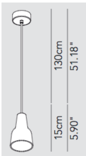
Product Name: Eva Mini Designer: Hans Thyge Raunkjaer Manufacturer: Modo IP: 20 Light Source: GU10 20W max or Gu10 LED Material: Ceramic or Terracotta Finishes: White or Dark Brown
