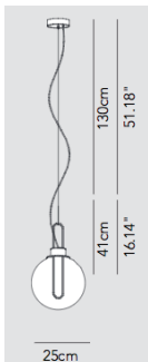
Product Name: Orb Designer: Büro Famos Manufacturer: Modo IP: 20 Light Source: LED 7W 3000K Material: PMMA / Metal Finishes: White, Black, Chrome, Copper, Brass
